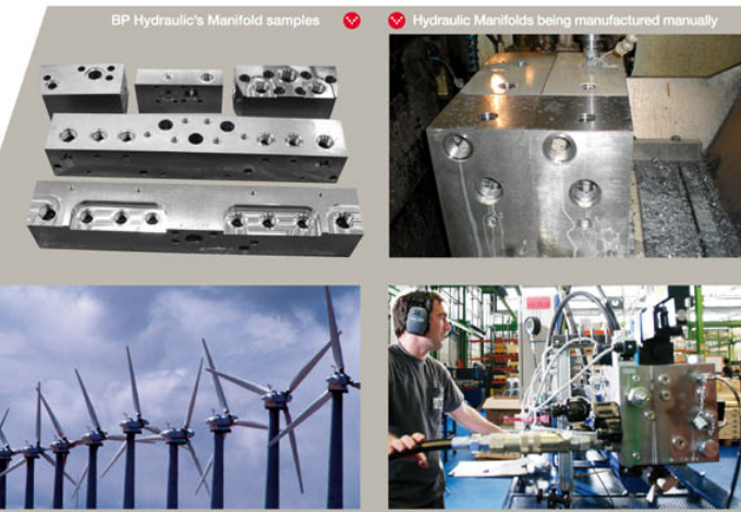
BP Hydraulic's Manifold samples ✓ ✓ Hydraulic Manifolds being manufactured manually ✓ Hydraulic Manifolds are main parts of Wind Turbines ✓ ✓ Hydraulic Manifold assembly for Wind Turbines ✓
